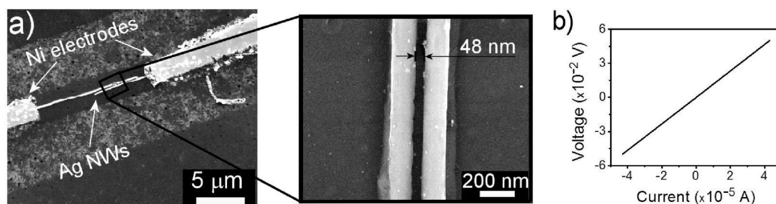
Figure 4. (a) SEM images of two parallel NWs, individually contacted with Ni electrodes and covered with a RG-O/Au NP film, used to measure the resistance of the system. Inset shows a higher magnification image showing the distance of 48 nm between the parallel Ag NWs (see also Figure S4 in Supporting Information). (b) I – V characteristic of the system.
