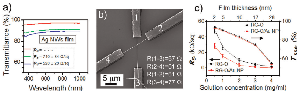
Figure 1. (a) R_s and T of Ag NW films obtained using three different concentrations of the Ag NW dispersions: (red) 1.0 mg/mL, (green) 2.0 mg/mL, and (blue) 2.5 mg/mL. (b) SEM image of a NW–NW junction with four Ni electrodes used to measure the resistance of individual NWs and the junction resistance between NWs. (c) R_s and T of RG-O and RG-O/Au NP films obtained by spin coating of the G-O and G-O/Au NP dispersions with different concentrations and then exposing the films to hydrazine vapor at 100 ^{\circ}\text{C} .
